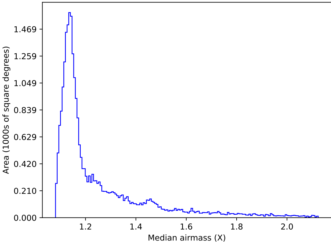
early_u_fpextra4.0_v3.4_10yrs All sky i band: Median airmass
