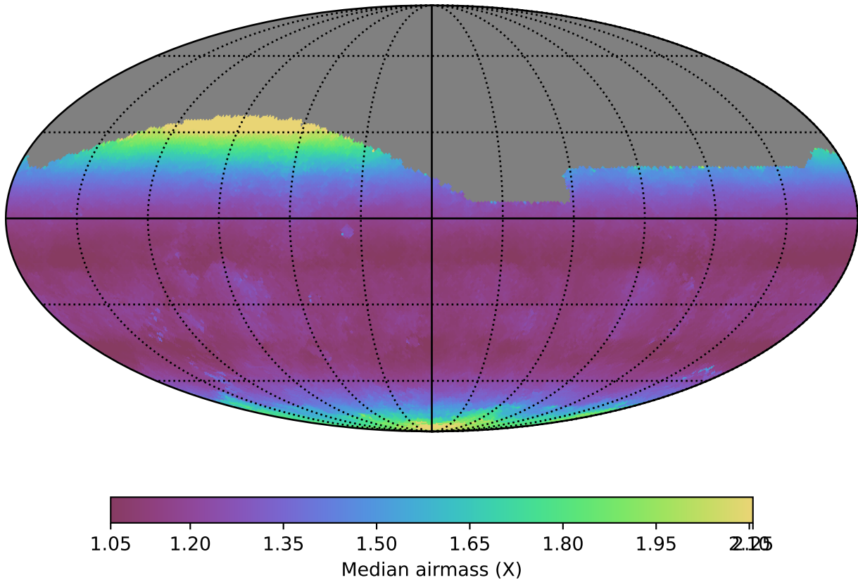
early_u_fpextra4.0_v3.4_10yrs All sky g band: Median airmass
