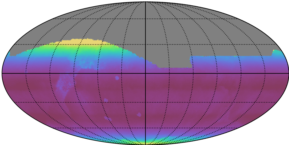
early_u_fpextra4.0_v3.4_10yrs All sky all bands: Median airmass
