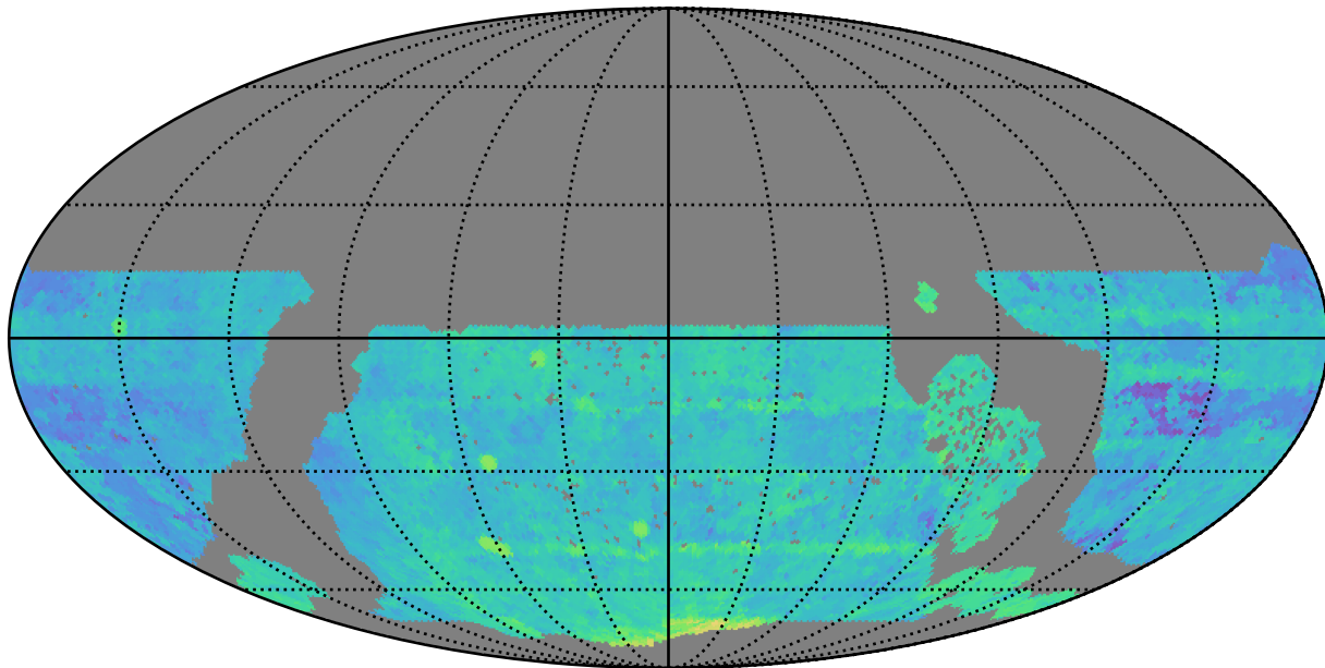
early_u_fpextra4.0_v3.4_10yrs WFD i band: Median Season Length
