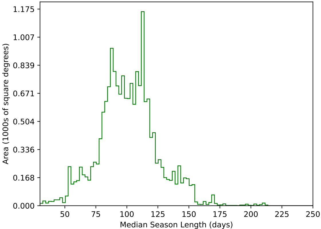
early_u_fpextra4.0_v3.4_10yrs WFD g band: Median Season Length
