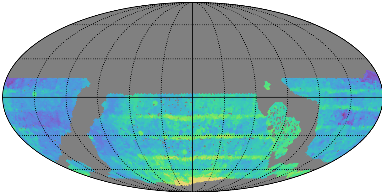
early_u_fpextra4.0_v3.4_10yrs WFD all bands: Median Season Length
