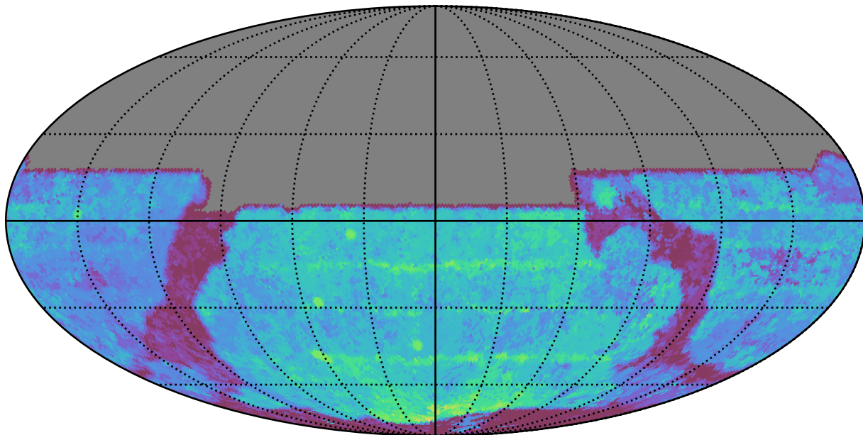
early_u_fpextra4.0_v3.4_10yrs All sky y band: Median Season Length
