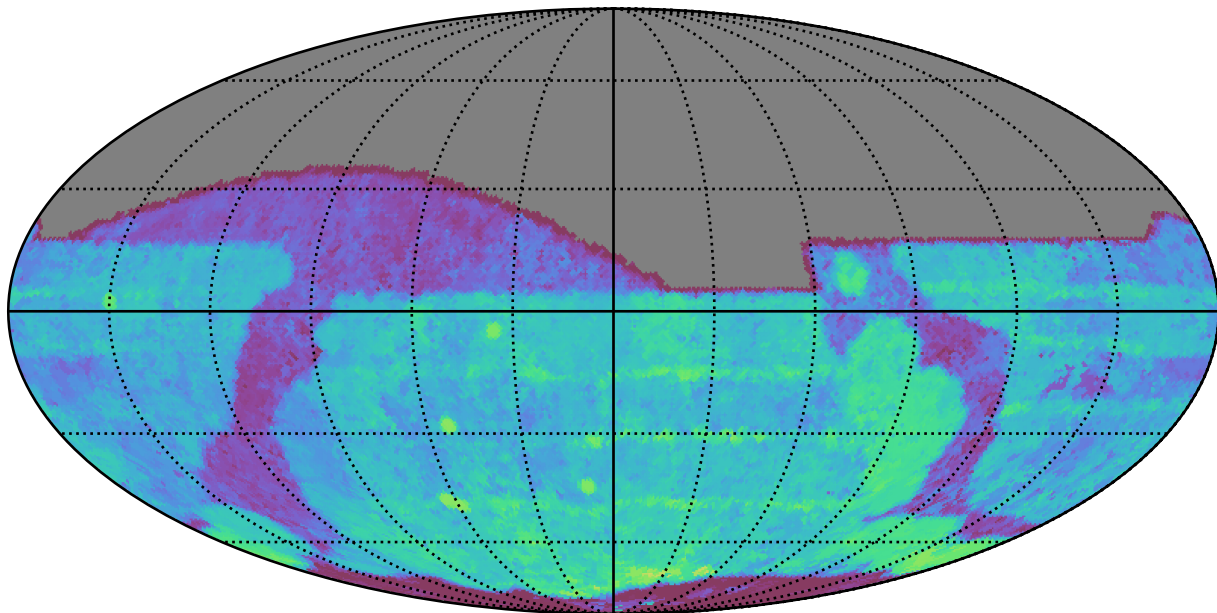
early_u_fpextra4.0_v3.4_10yrs All sky r band: Median Season Length
