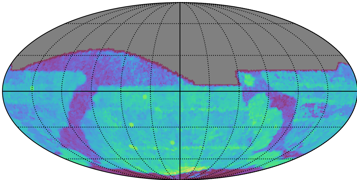
early_u_fpextra4.0_v3.4_10yrs All sky i band: Median Season Length
