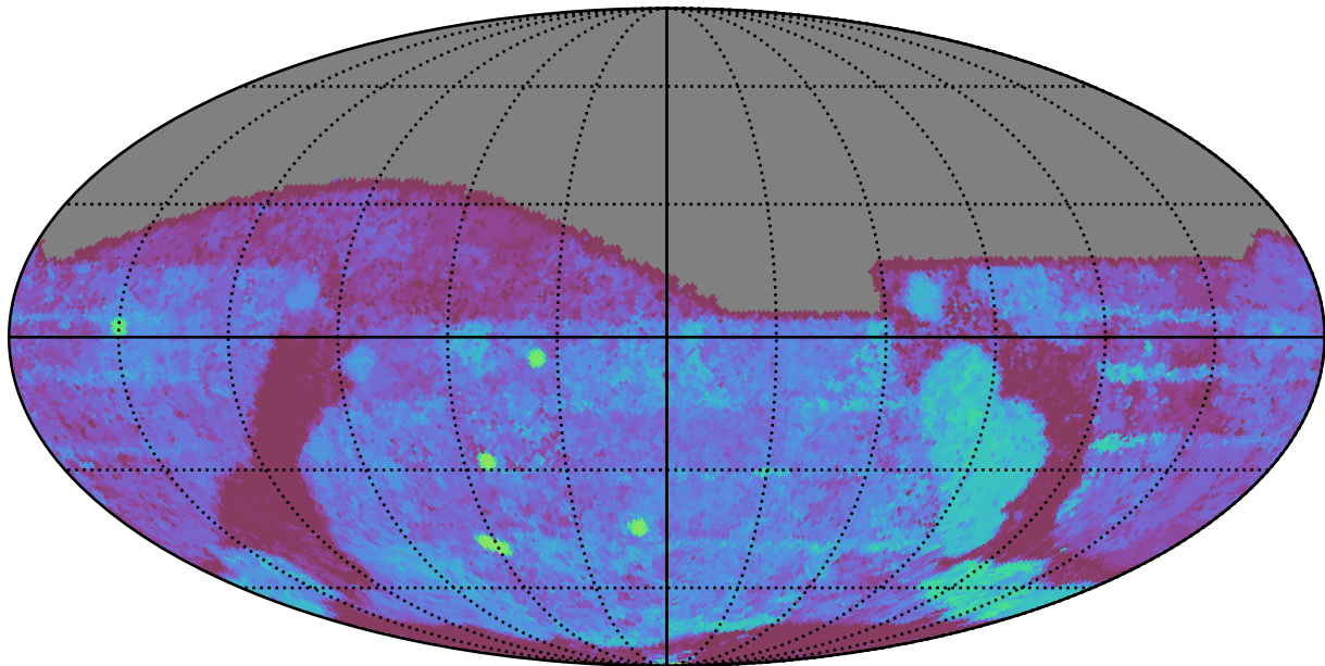
early_u_fpextra4.0_v3.4_10yrs All sky g band: Median Season Length
