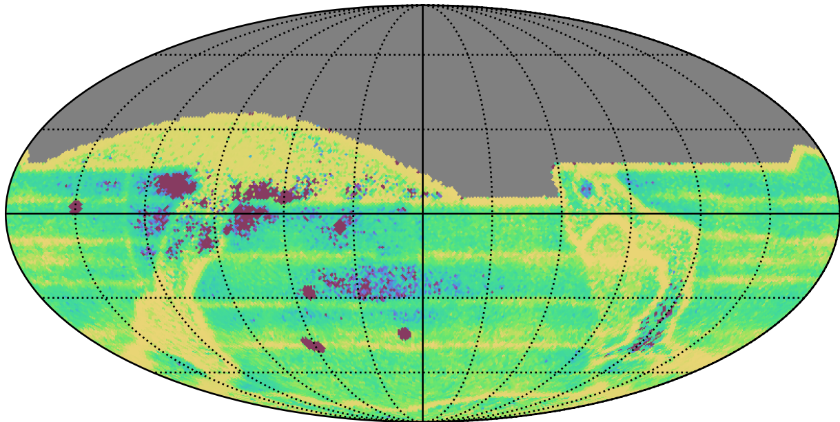
early_u_fpextra4.0_v3.4_10yrs All sky: Median Intra-Night Gap
