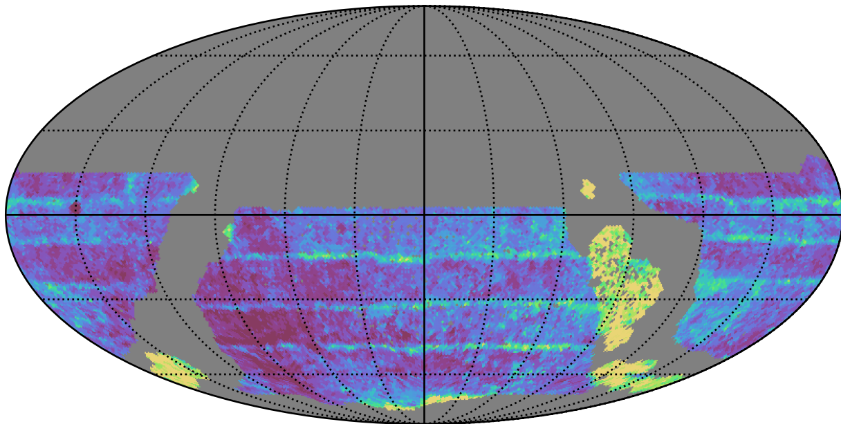
early_u_fpextra4.0_v3.4_10yrs WFD z band: Median Inter-Night Gap
