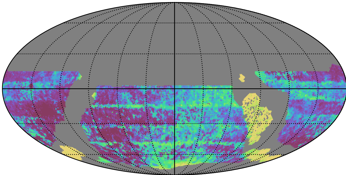
early_u_fpextra4.0_v3.4_10yrs WFD y band: Median Inter-Night Gap
