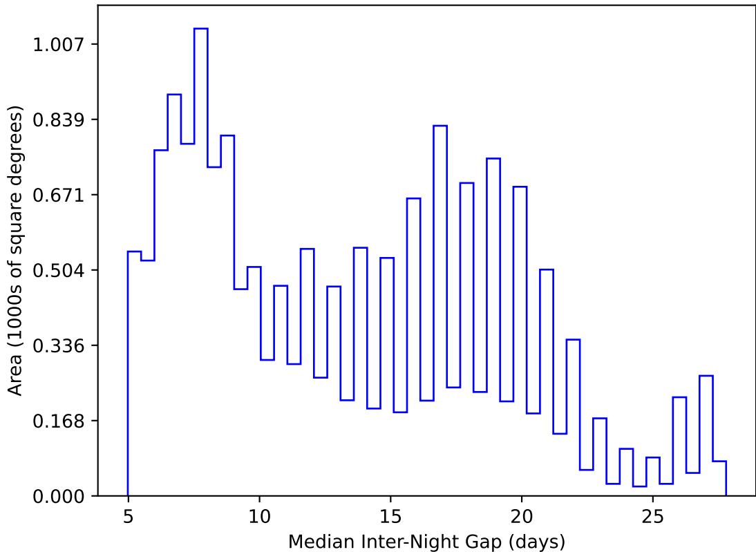
early_u_fpextra4.0_v3.4_10yrs WFD y band: Median Inter-Night Gap
