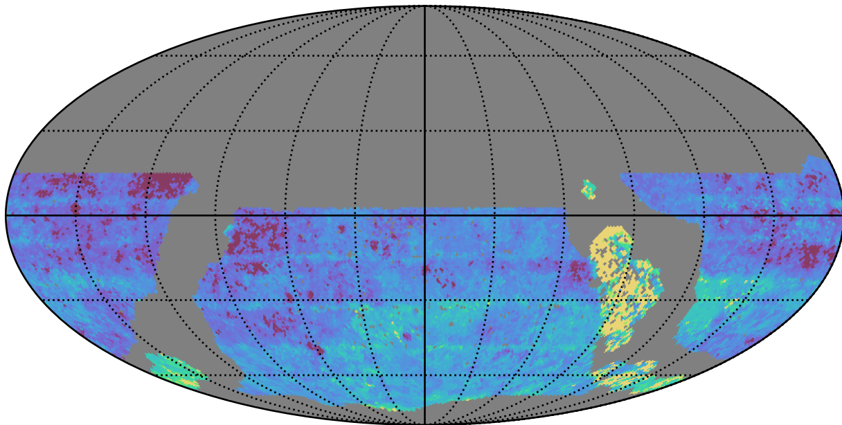
early_u_fpextra4.0_v3.4_10yrs WFD u band: Median Inter-Night Gap
