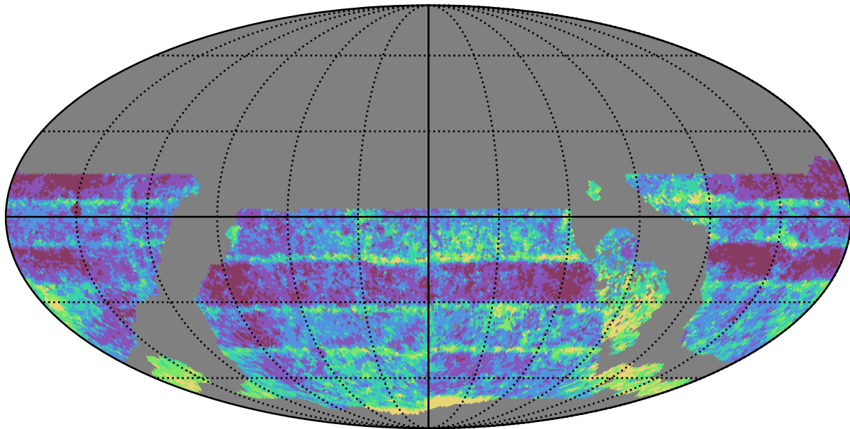
early_u_fpextra4.0_v3.4_10yrs WFD r band: Median Inter-Night Gap
