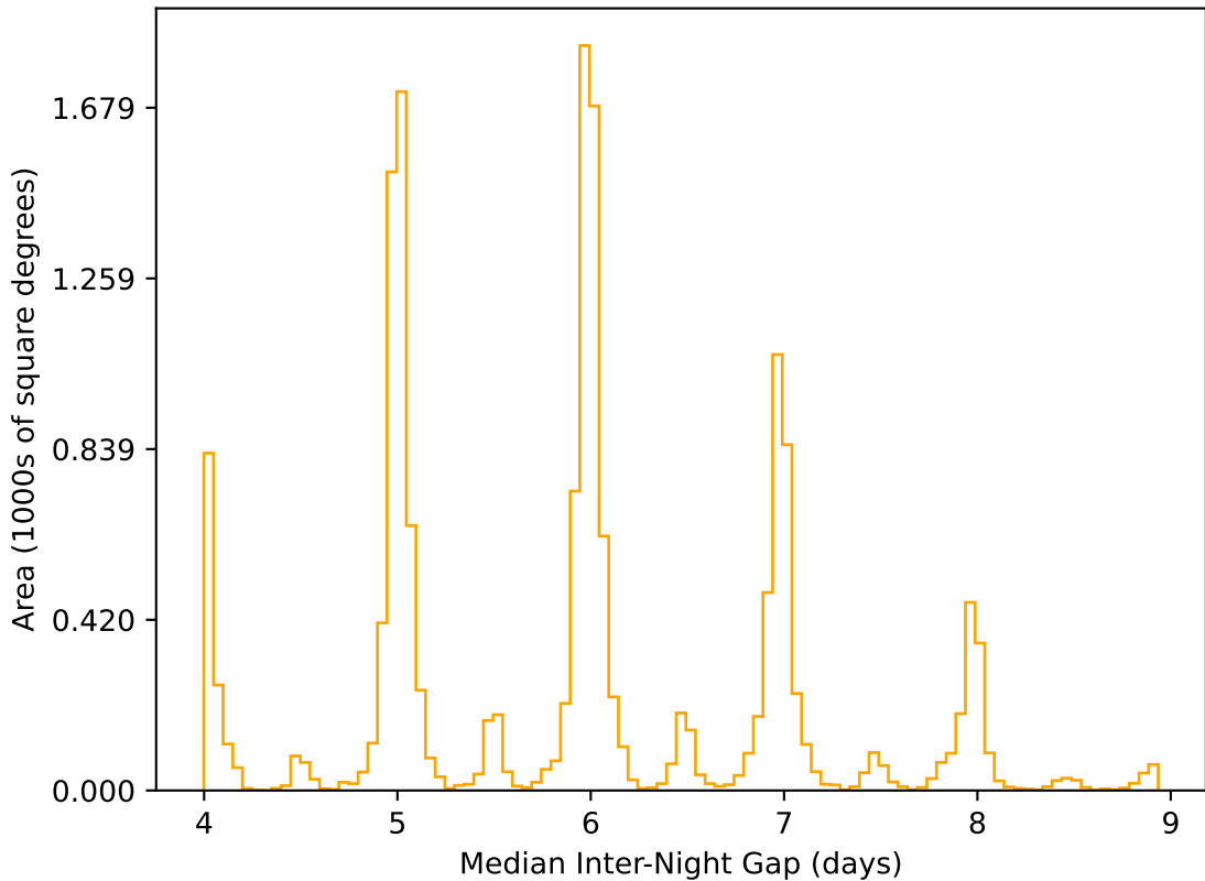
early_u_fpextra4.0_v3.4_10yrs WFD r band: Median Inter-Night Gap
