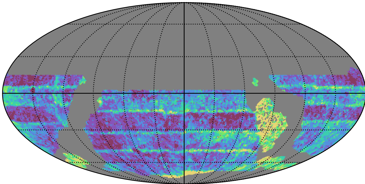
early_u_fpextra4.0_v3.4_10yrs WFD i band: Median Inter-Night Gap
