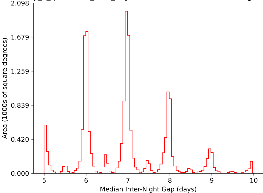
early_u_fpextra4.0_v3.4_10yrs WFD i band: Median Inter-Night Gap
