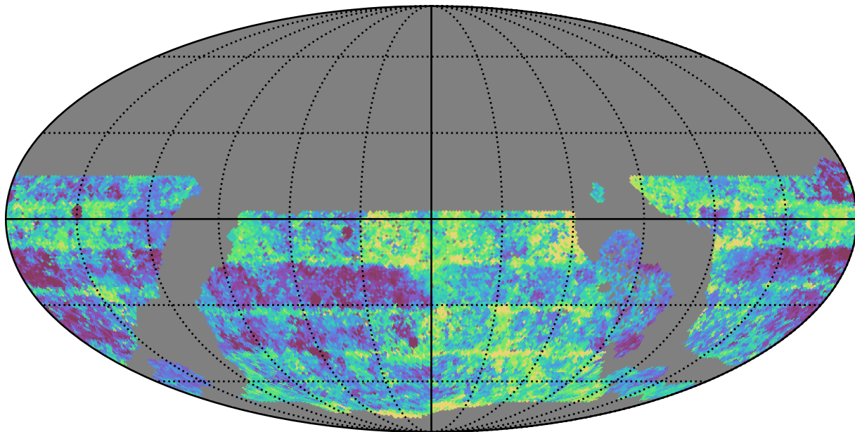
early_u_fpextra4.0_v3.4_10yrs WFD g band: Median Inter-Night Gap
