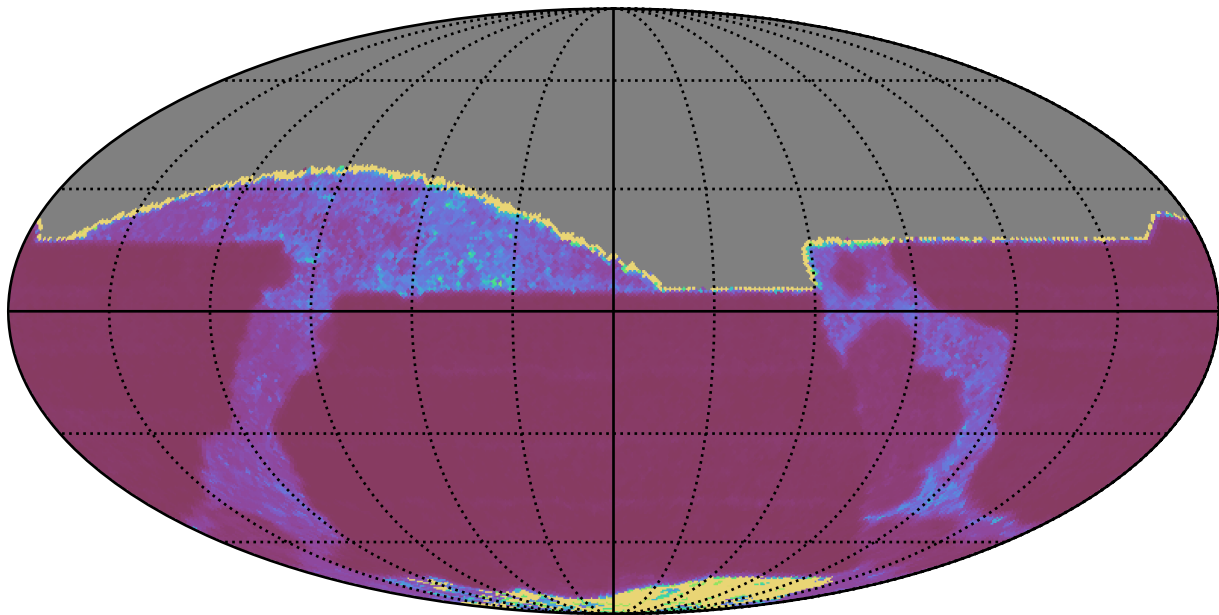
early_u_fpextra4.0_v3.4_10yrs All sky z band: Median Inter-Night Gap
