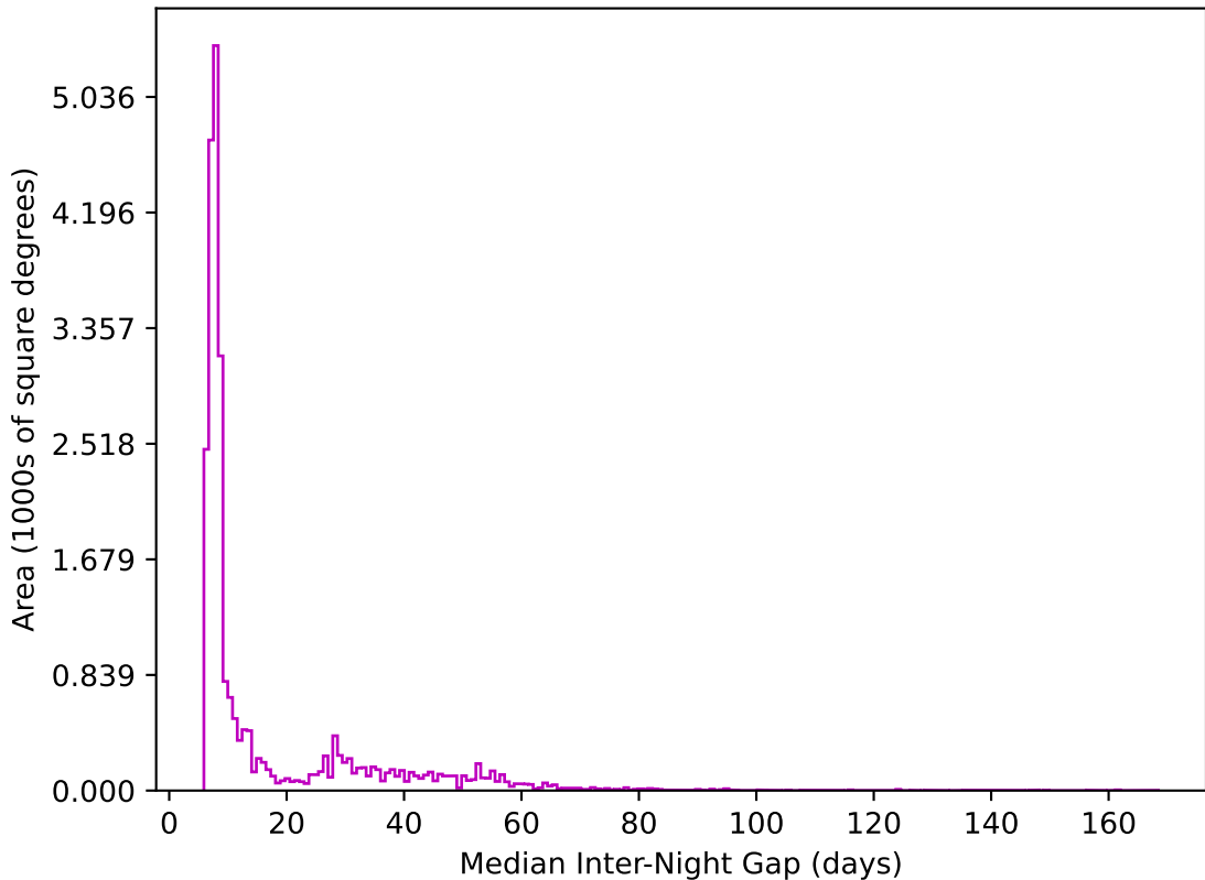
early_u_fpextra4.0_v3.4_10yrs All sky z band: Median Inter-Night Gap
