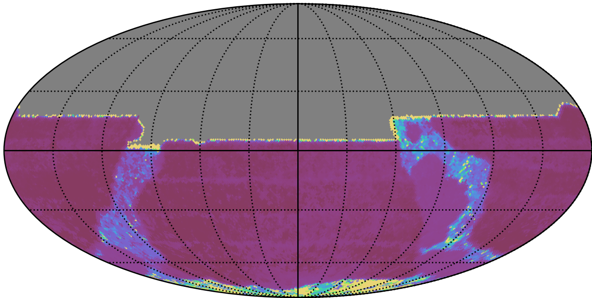
early_u_fpextra4.0_v3.4_10yrs All sky y band: Median Inter-Night Gap
