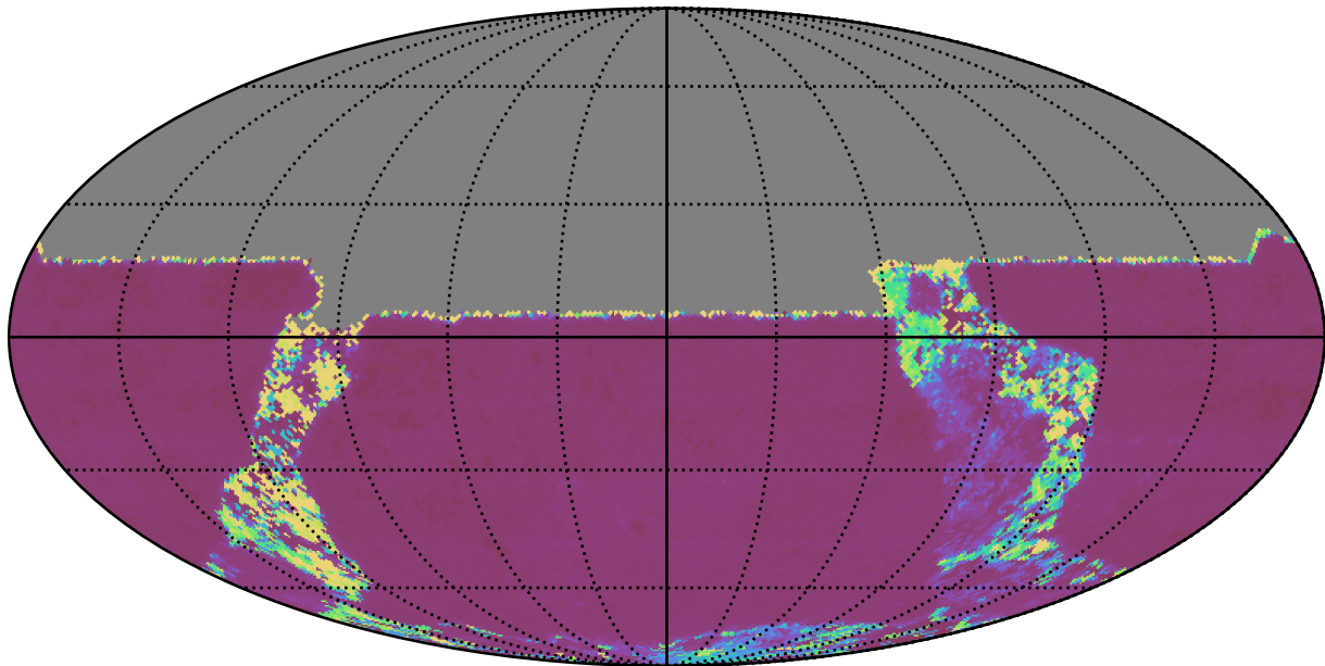
early_u_fpextra4.0_v3.4_10yrs All sky u band: Median Inter-Night Gap
