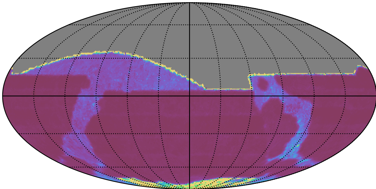
early_u_fpextra4.0_v3.4_10yrs All sky r band: Median Inter-Night Gap
