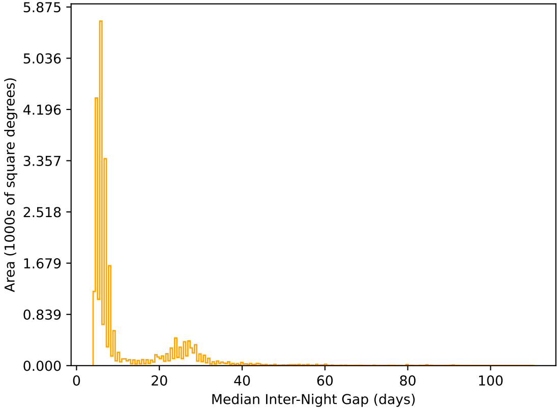
early_u_fpextra4.0_v3.4_10yrs All sky r band: Median Inter-Night Gap
