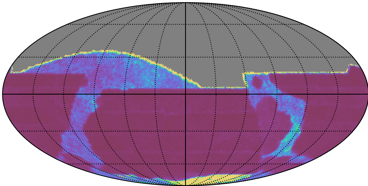
early_u_fpextra4.0_v3.4_10yrs All sky i band: Median Inter-Night Gap
