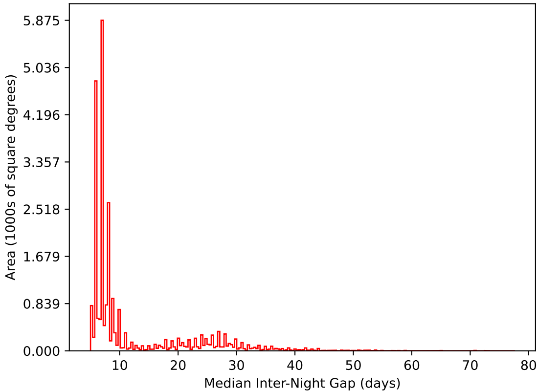
early_u_fpextra4.0_v3.4_10yrs All sky i band: Median Inter-Night Gap
