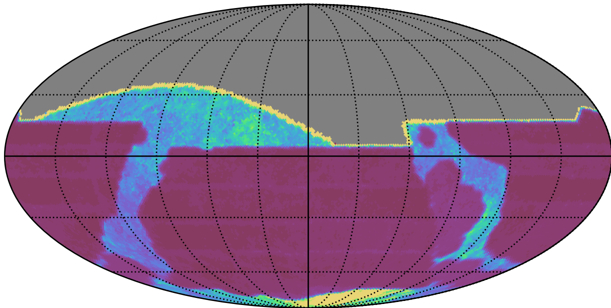
early_u_fpextra4.0_v3.4_10yrs All sky all bands: Median Inter-Night Gap
