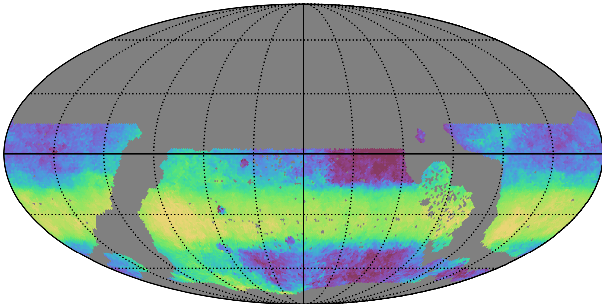
early_u_fpextra4.0_v3.4_10yrs WFD y band: Median HA
