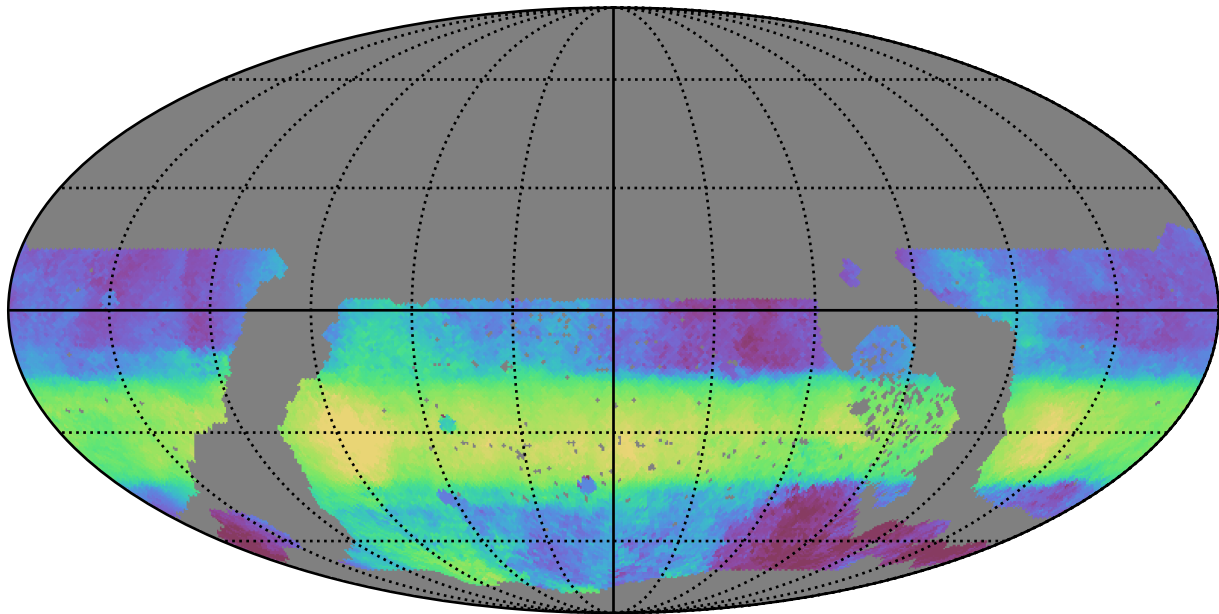
early_u_fpextra4.0_v3.4_10yrs WFD r band: Median HA
