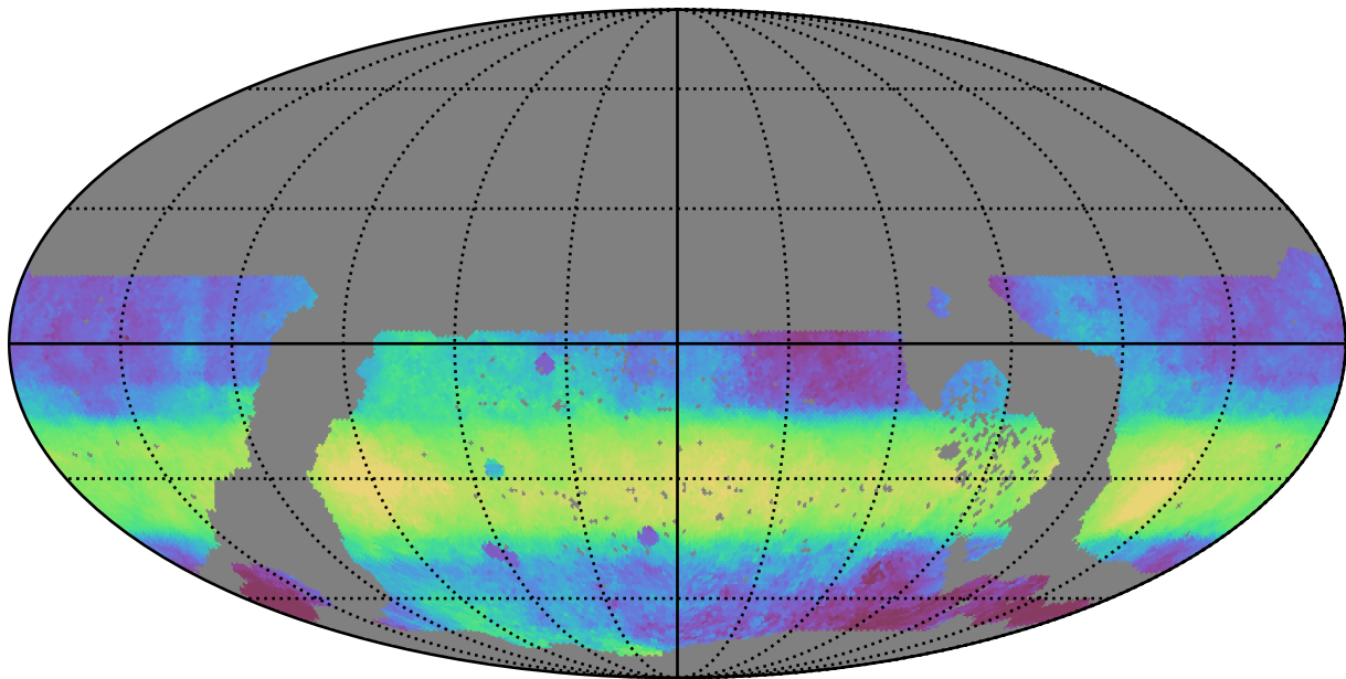
early_u_fpextra4.0_v3.4_10yrs WFD i band: Median HA
