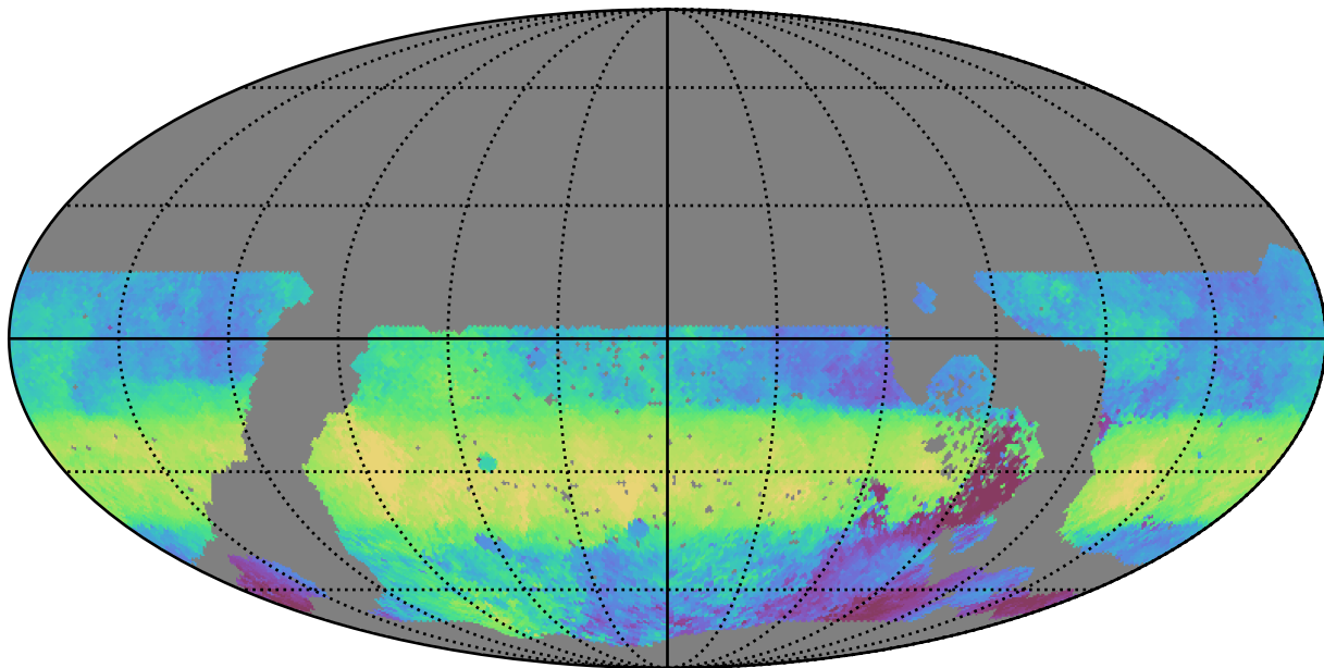
early_u_fpextra4.0_v3.4_10yrs WFD g band: Median HA
