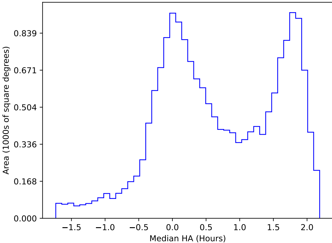
early_u_fpextra4.0_v3.4_10yrs WFD g band: Median HA
