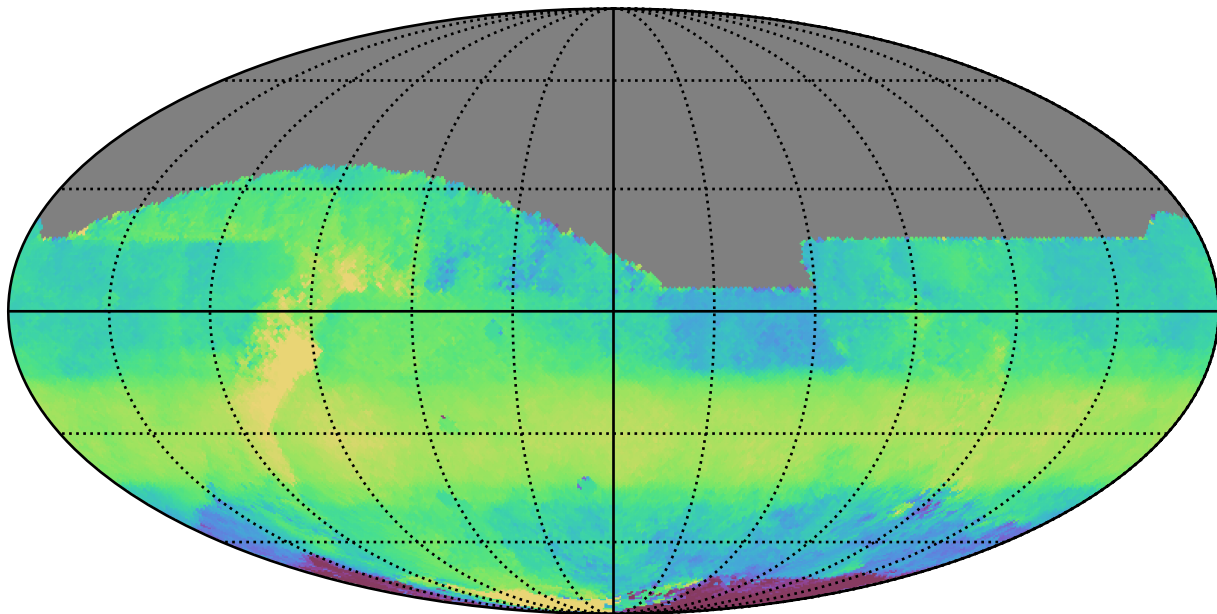
early_u_fpextra4.0_v3.4_10yrs All sky z band: Median HA
