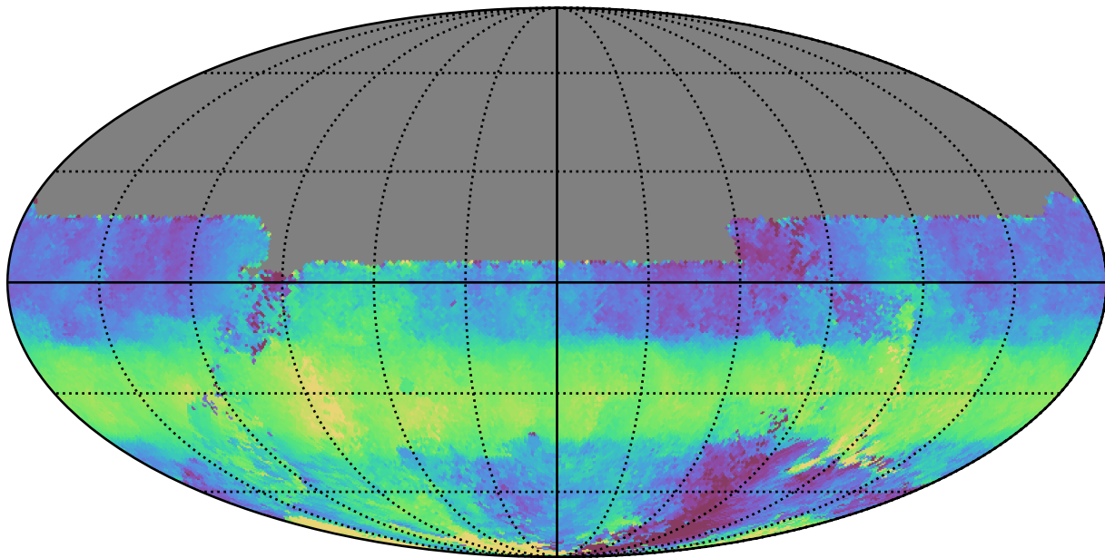
early_u_fpextra4.0_v3.4_10yrs All sky u band: Median HA
