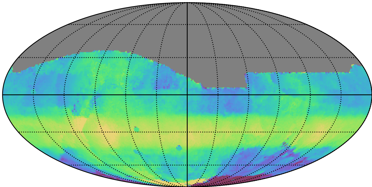
early_u_fpextra4.0_v3.4_10yrs All sky r band: Median HA
