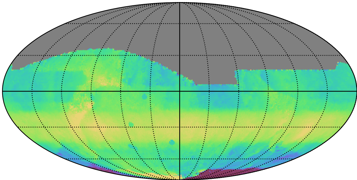
early_u_fpextra4.0_v3.4_10yrs All sky i band: Median HA
