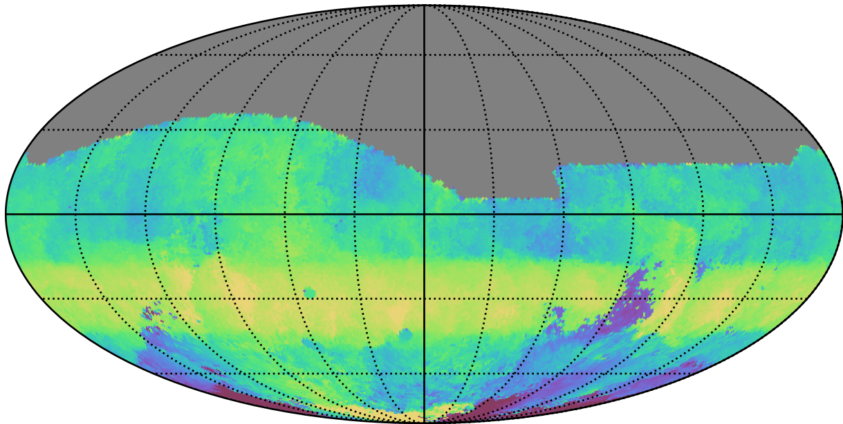
early_u_fpextra4.0_v3.4_10yrs All sky g band: Median HA
