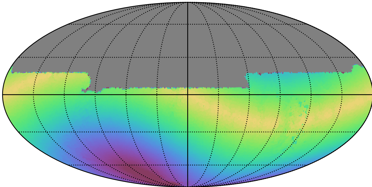
early_u_fpextra4.0_v3.4_10yrs All sky u band: Max solarElong
