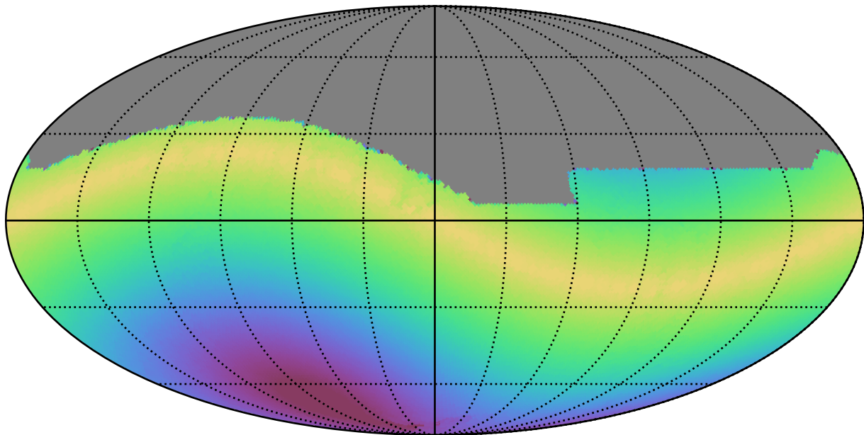
early_u_fpextra4.0_v3.4_10yrs All sky r band: Max solarElong
