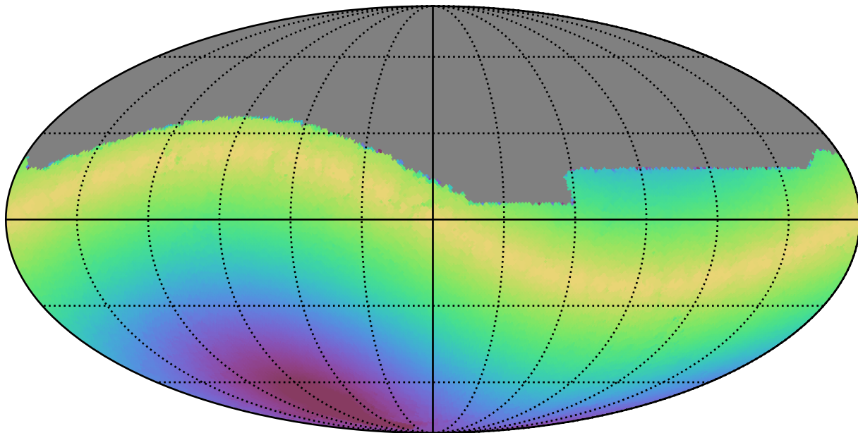
early_u_fpextra4.0_v3.4_10yrs All sky g band: Max solarElong
