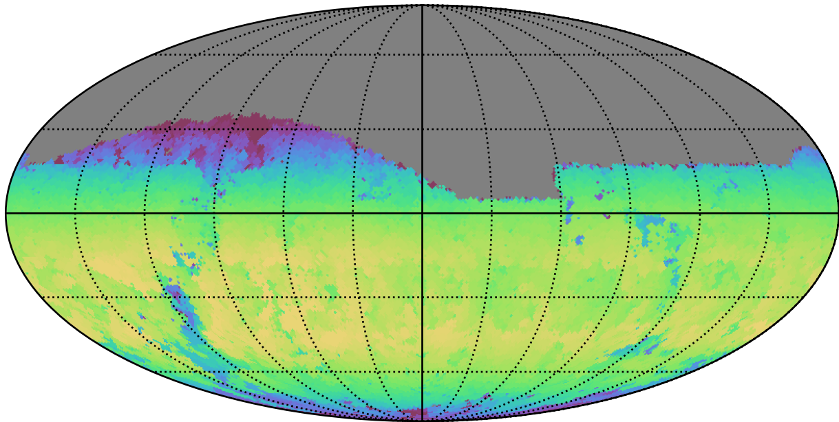
early_u_fpextra4.0_v3.4_10yrs Yr 1 z band: Max skyBrightness
