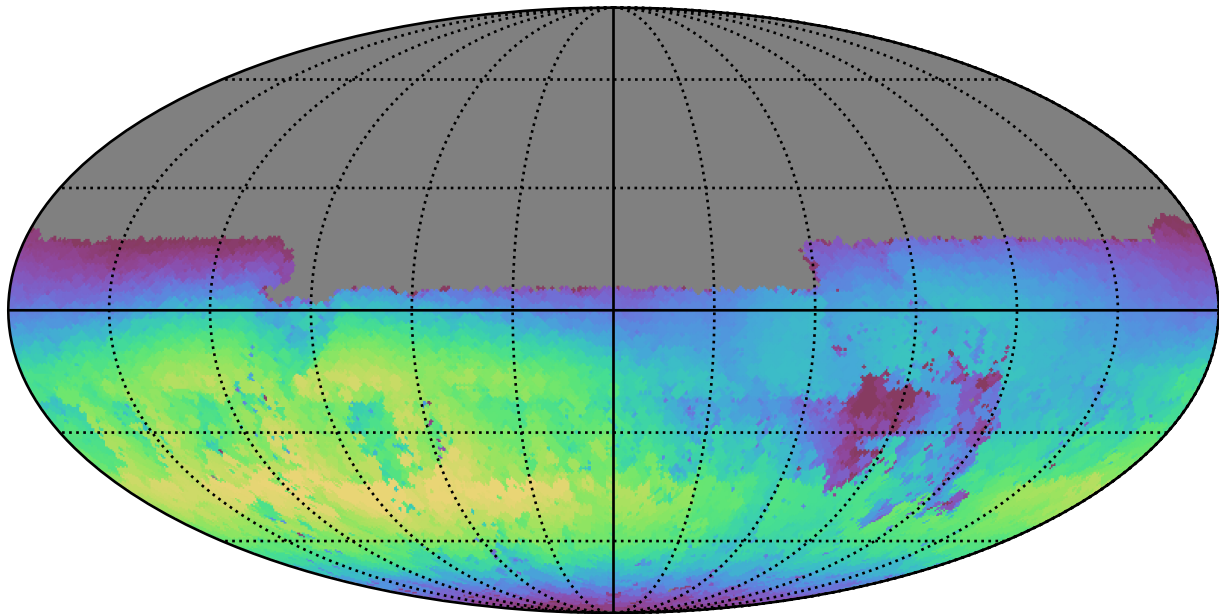
early_u_fpextra4.0_v3.4_10yrs Yr 1 u band: Max skyBrightness
