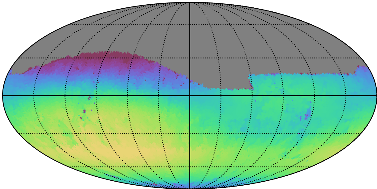
early_u_fpextra4.0_v3.4_10yrs Yr 1 r band: Max skyBrightness
