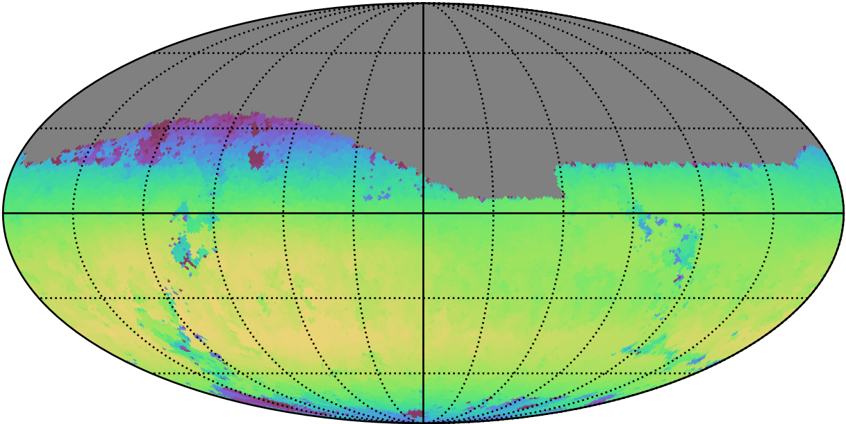
early_u_fpextra4.0_v3.4_10yrs Yr 1 i band: Max skyBrightness
