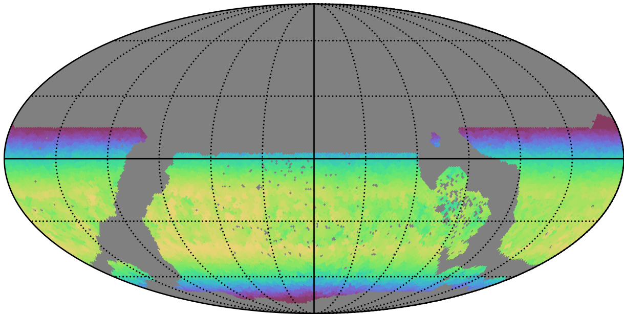
early_u_fpextra4.0_v3.4_10yrs WFD y band: Max skyBrightness
