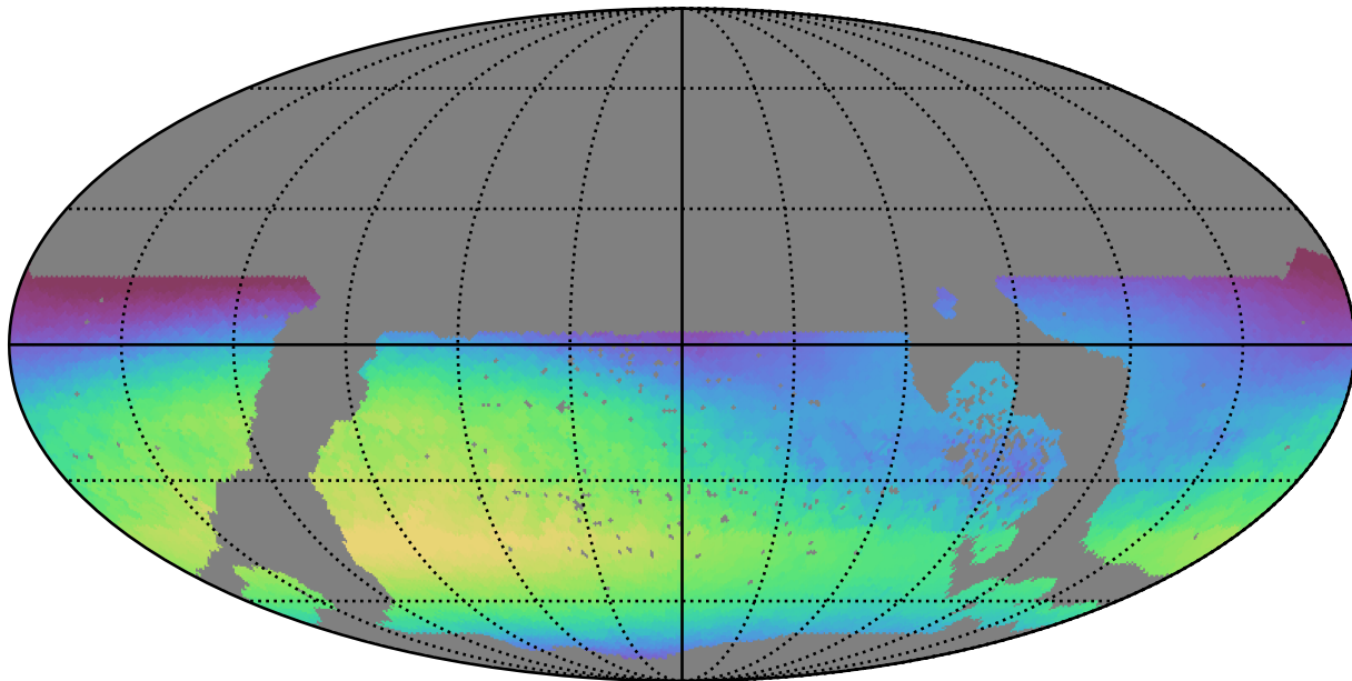
early_u_fpextra4.0_v3.4_10yrs WFD u band: Max skyBrightness
