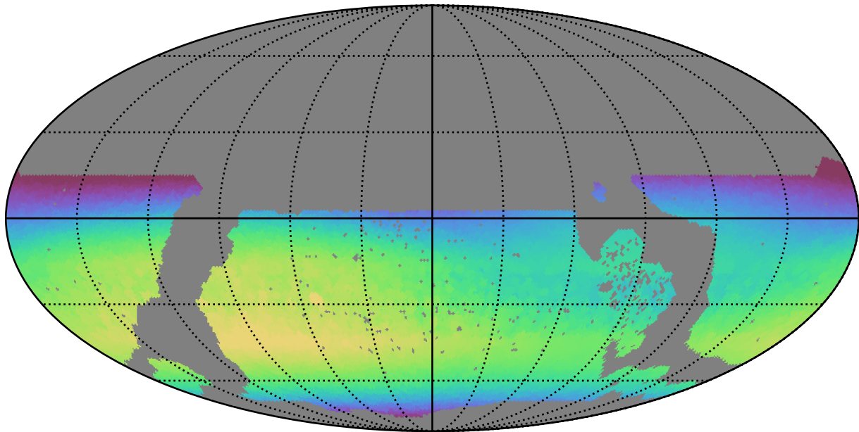
early_u_fpextra4.0_v3.4_10yrs WFD i band: Max skyBrightness
