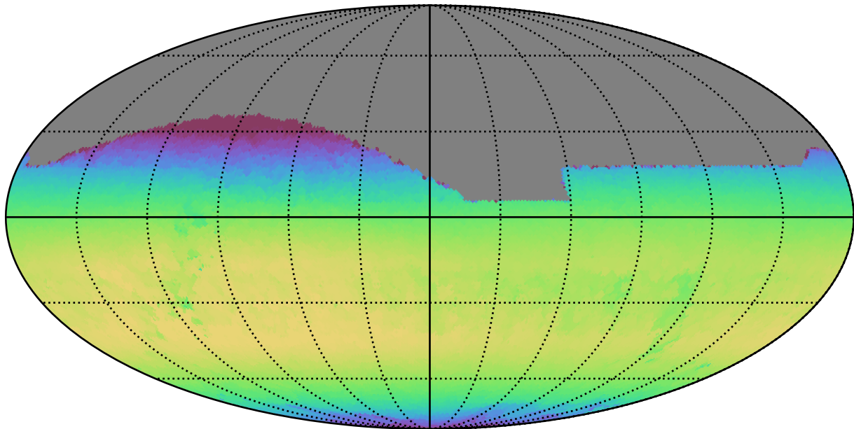
early_u_fpextra4.0_v3.4_10yrs All sky z band: Max skyBrightness
